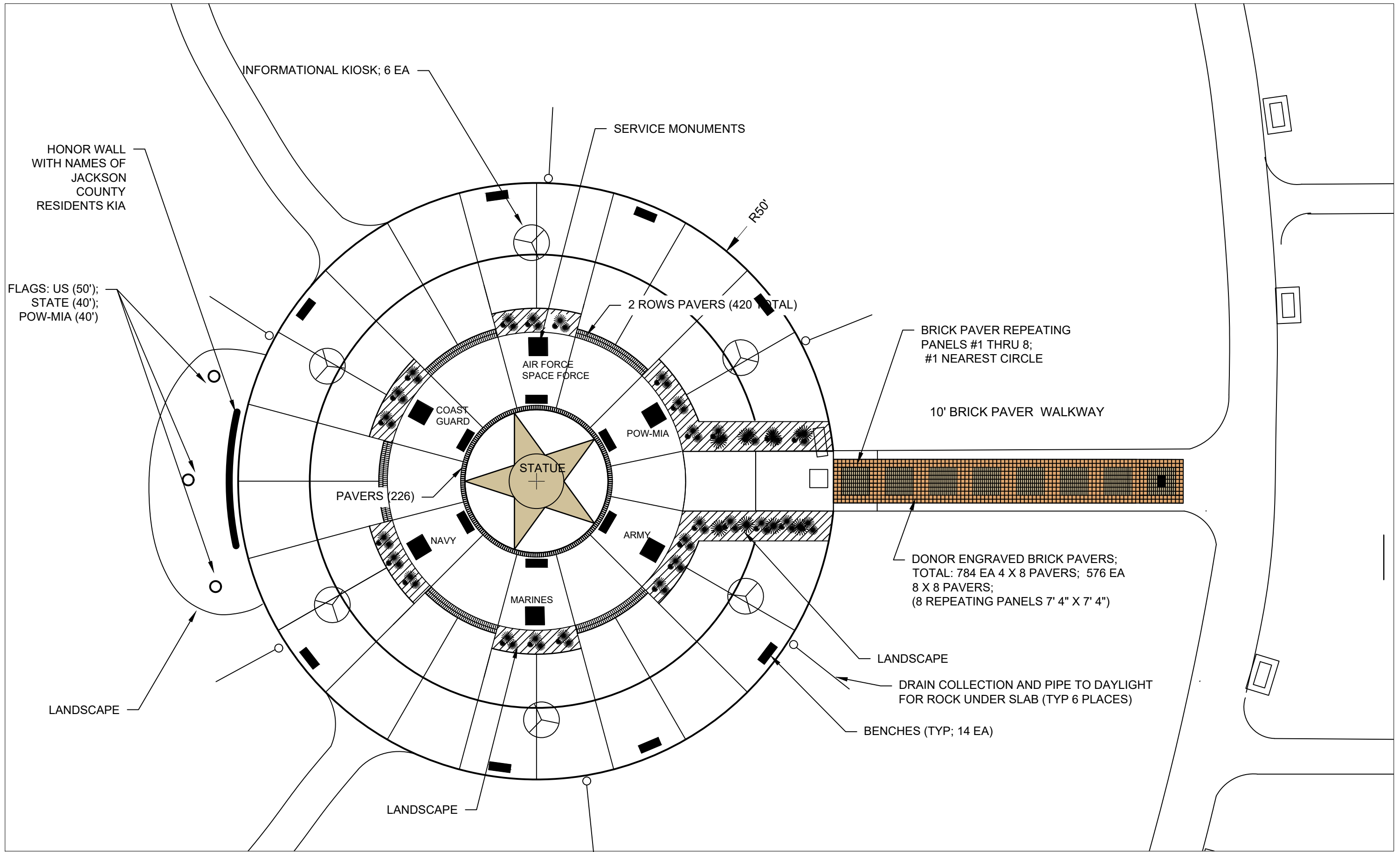
PLAN 1" = 15'
